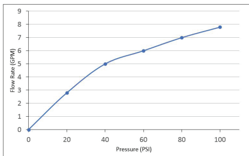
V-2316B Flow Rate (GPM) Vs Pressure (PSI) For Tub Port*
